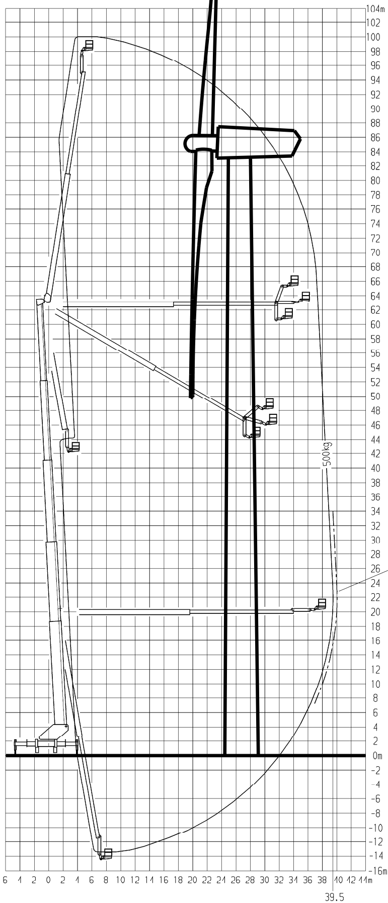
Turbine Access Diagram
